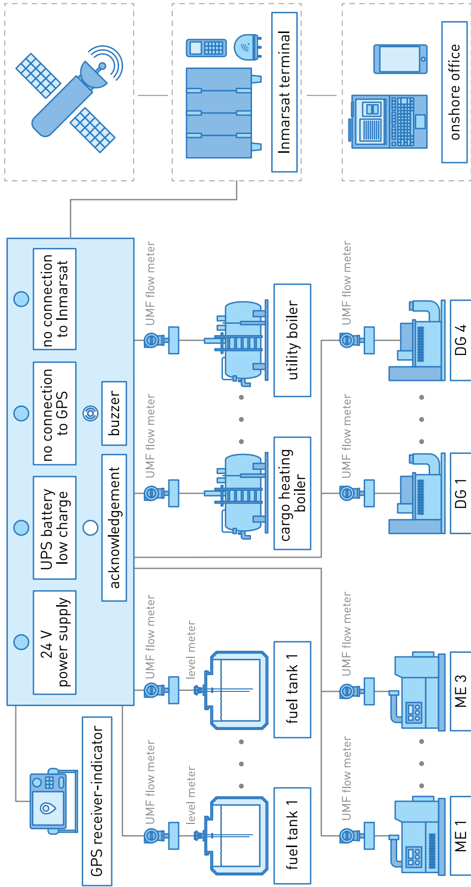
Block diagram of the fuel consumption monitoring system
